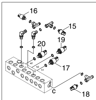
SHUTTLE BLOCK
